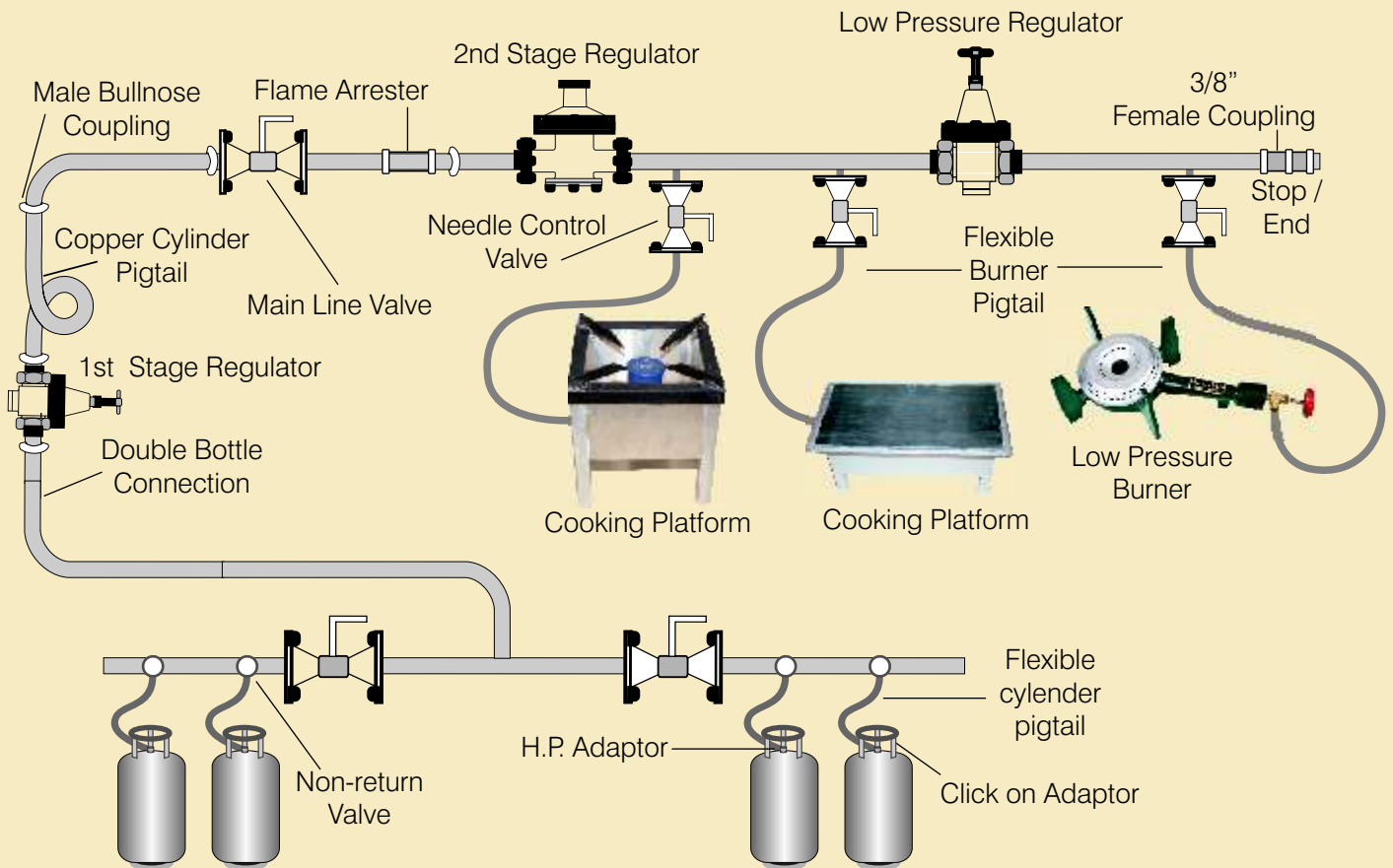
SCHEMATIC DIAGRAM TO SHOW AN IDEAL INSTALLATION (COMMERCIAL)
