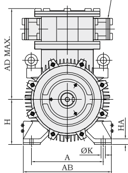
LF-180 to LF-225 Frame Gas Group I/IIA/IIB
