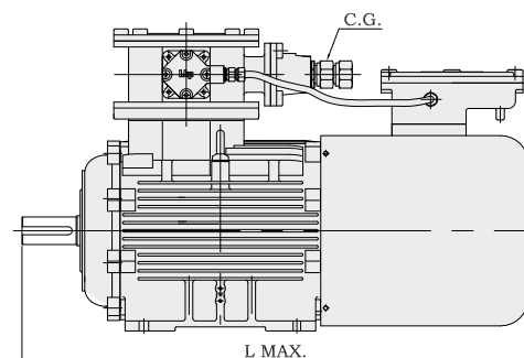
BRAKE MOTOR (DIMENSION NOMANCLATURE SIMILAR TO FLP STANDARD MOTOR) For Gas Group IIA & IIB
