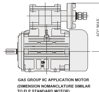
LF-90 to LF-315 Frame Gas Group IIC
