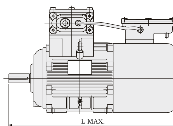
BRAKE MOTOR (DIMENSION NOMANCLATURE SIMILAR TO FLP STANDARD MOTOR) For Gas Group I, IIA & IIB
