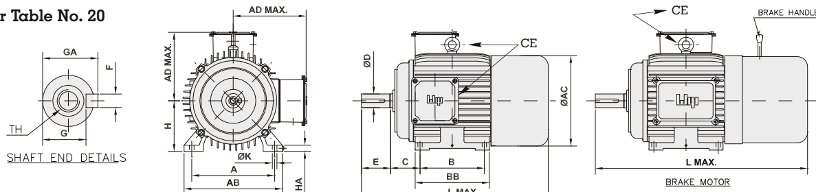
CE - Cable Entry in Metric
