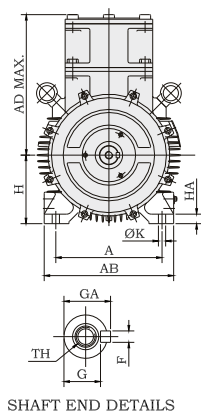
LF-90 to LF-160 Frame Gas Group I/IIA/IIB
