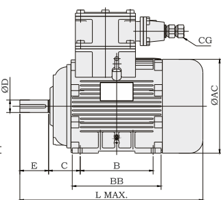
LF-90 to LF-160 Frame Gas Group I/IIA/IIB
